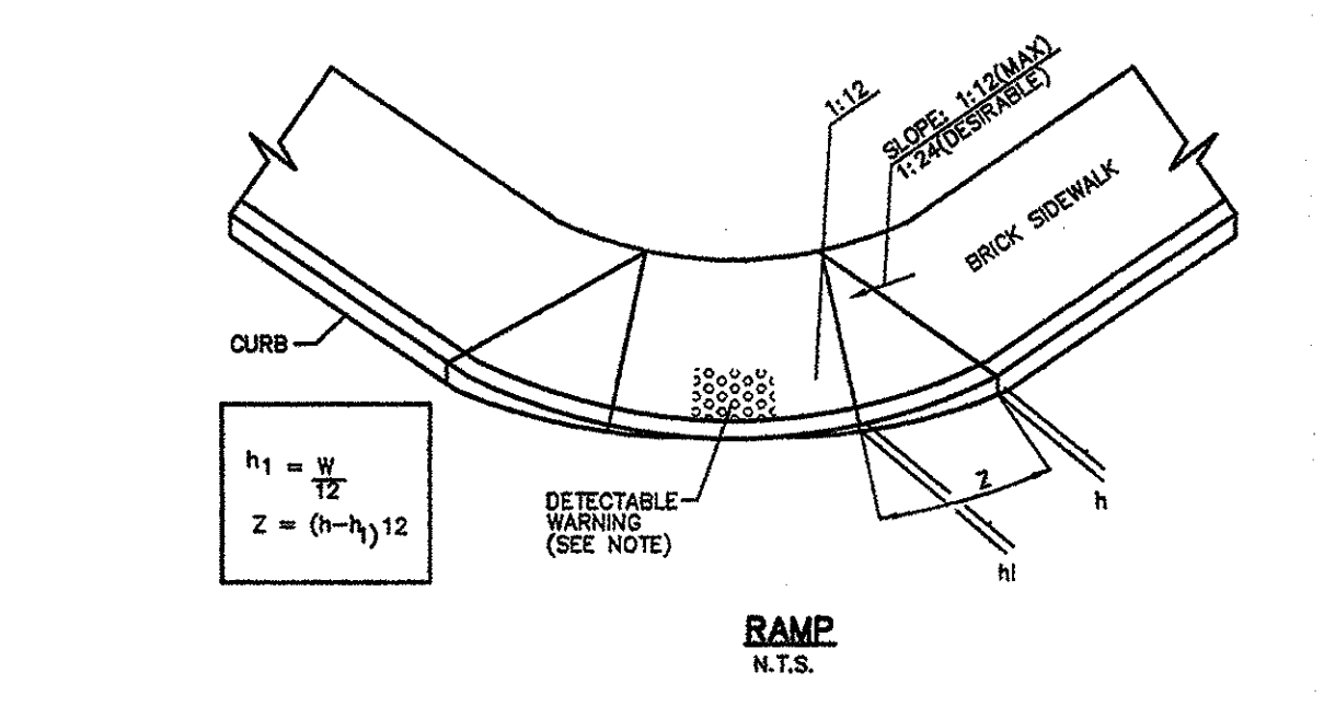
HANDICAPPED RAMP DETAILS N.T.S.
