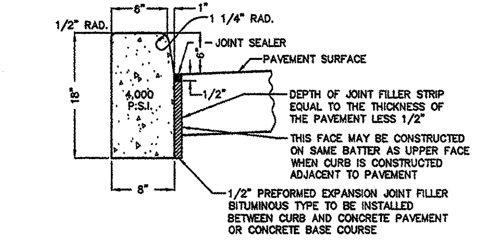
CITY CURB AND EXPANSION JOINT DETAIL N.T.S.
